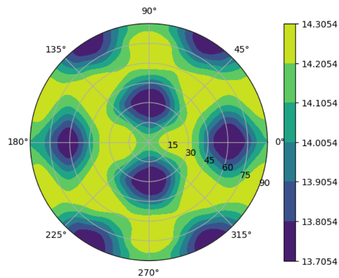
Figure 24: Directional resolution in the projection sphere.
