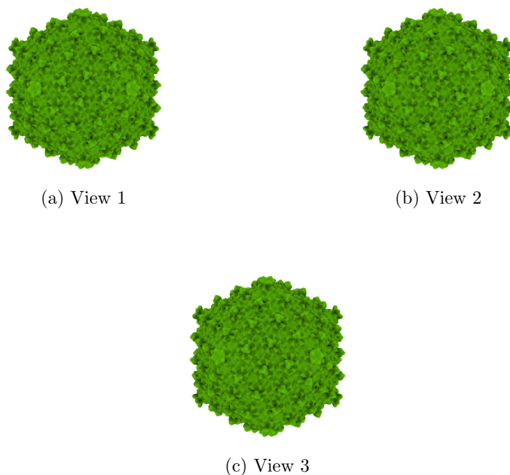
Figure 4: Isosurface at threshold=-500.000000. Views generated by ChimeraX at the following X, Y, Z angles: View 1 (0, -90, -90), View 2 (-90, 0, -90), View 3 (0, 0, 0).
