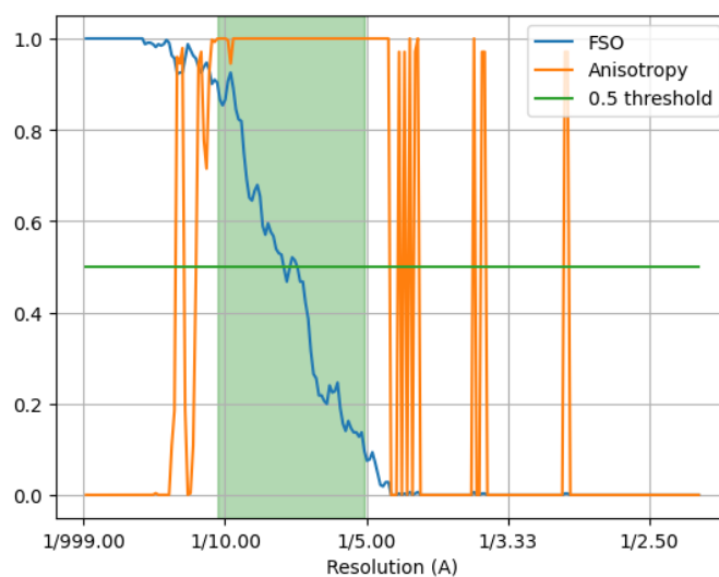
Figure 25: FSO and anisotropy.
