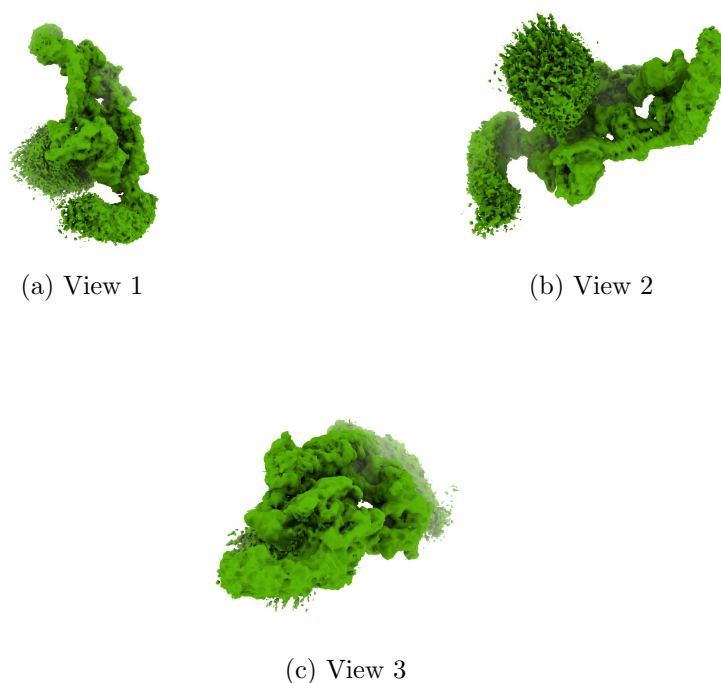
Figure 4: Isosurface at threshold=0.217000. Views generated by ChimeraX at a the following X, Y, Z angles: View 1 (0, -90, -90), View 2 (-90, 0, -90), View 3 (0, 0, 0).
