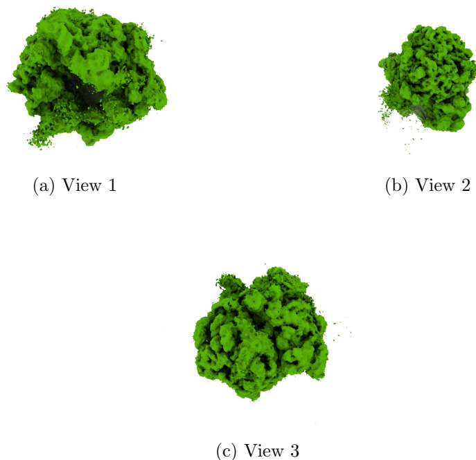
Figure 4: Isosurface at threshold=0.447000. Views generated by ChimeraX at a the following X, Y, Z angles: View 1 (0, -90, -90), View 2 (-90, 0, -90), View 3 (0, 0, 0).
