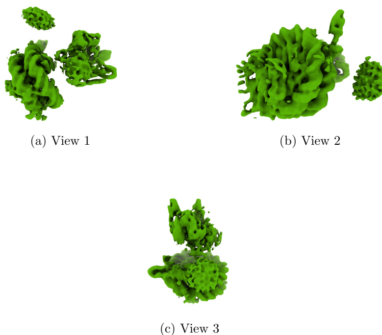
Figure 4: Isosurface at threshold=0.027500. Views generated by ChimeraX at a the following X, Y, Z angles: View 1 (0, -90, -90), View 2 (-90, 0, -90), View 3 (0, 0, 0).
