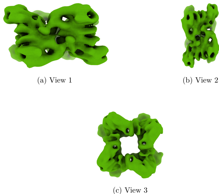
Figure 4: Isosurface at threshold=0.032500. Views generated by ChimeraX at a the following X, Y, Z angles: View 1 (0, -90, -90), View 2 (-90, 0, -90), View 3 (0, 0, 0).
