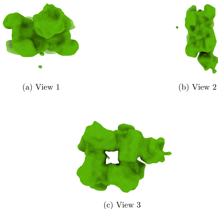
Figure 4: Isosurface at threshold=0.014600. Views generated by ChimeraX at a the following X, Y, Z angles: View 1 (0, -90, -90), View 2 (-90, 0, -90), View 3 (0, 0, 0).
