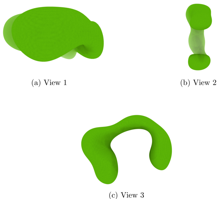
Figure 4: Isosurface at threshold=0.800000. Views generated by ChimeraX at the following X, Y, Z angles: View 1 (0, -90, -90), View 2 (-90, 0, -90), View 3 (0, 0, 0).
