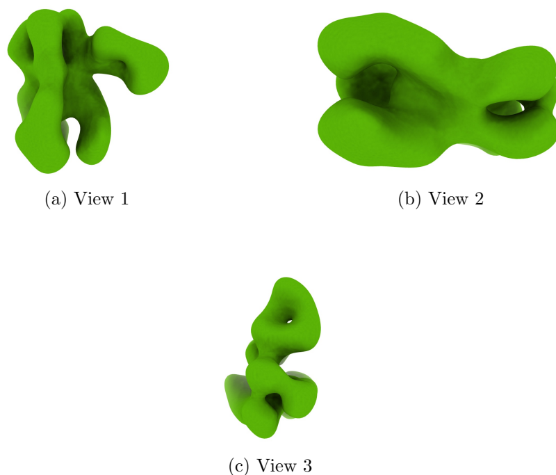
Figure 4: Isosurface at threshold=0.031400. Views generated by ChimeraX at a the following X, Y, Z angles: View 1 (0, -90, -90), View 2 (-90, 0, -90), View 3 (0, 0, 0).
