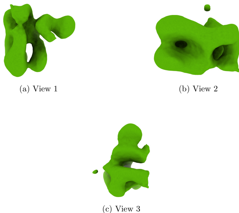
Figure 4: Isosurface at threshold=0.018600. Views generated by ChimeraX at a the following X, Y, Z angles: View 1 (0, -90, -90), View 2 (-90, 0, -90), View 3 (0, 0, 0).
