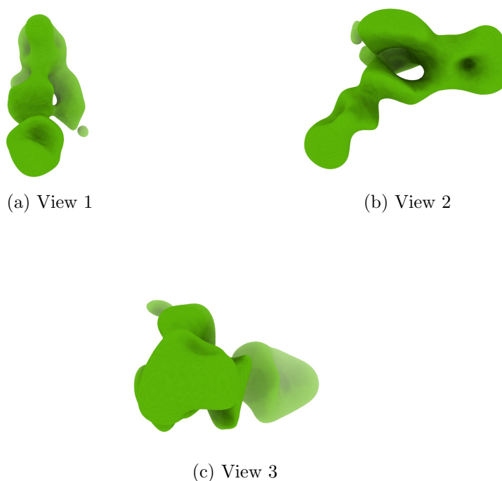
Figure 4: Isosurface at threshold=0.025700. Views generated by ChimeraX at a the following X, Y, Z angles: View 1 (0, -90, -90), View 2 (-90, 0, -90), View 3 (0, 0, 0).
