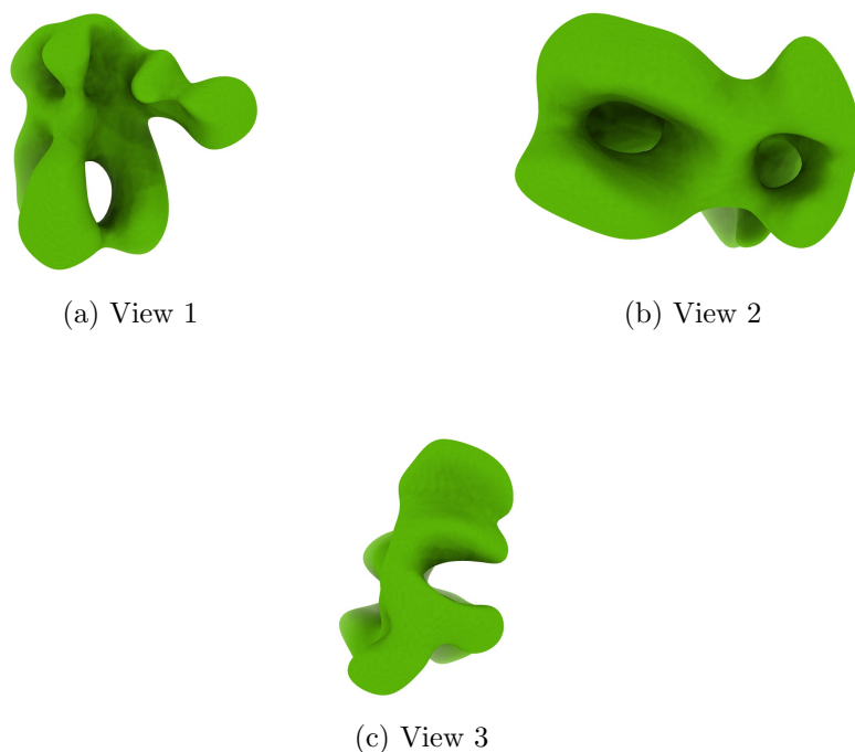
Figure 4: Isosurface at threshold=0.025700. Views generated by ChimeraX at a the following X, Y, Z angles: View 1 (0, -90, -90), View 2 (-90, 0, -90), View 3 (0, 0, 0).
