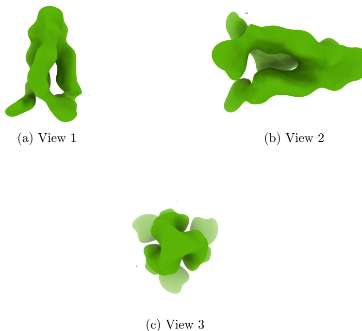
Figure 4: Isosurface at threshold=0.014600. Views generated by ChimeraX at a the following X, Y, Z angles: View 1 (0, -90, -90), View 2 (-90, 0, -90), View 3 (0, 0, 0).
