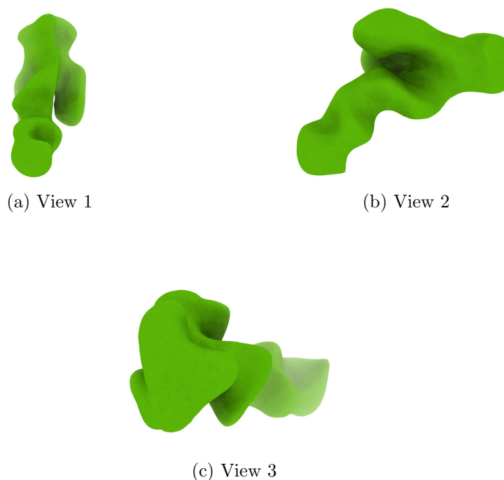
Figure 4: Isosurface at threshold=0.026200. Views generated by ChimeraX at a the following X, Y, Z angles: View 1 (0, -90, -90), View 2 (-90, 0, -90), View 3 (0, 0, 0).
