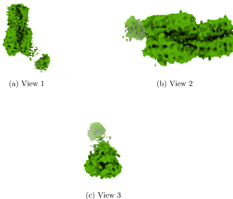
Figure 4: Isosurface at threshold=0.008100. Views generated by ChimeraX at a the following X, Y, Z angles: View 1 (0, -90, -90), View 2 (-90, 0, -90), View 3 (0, 0, 0).
