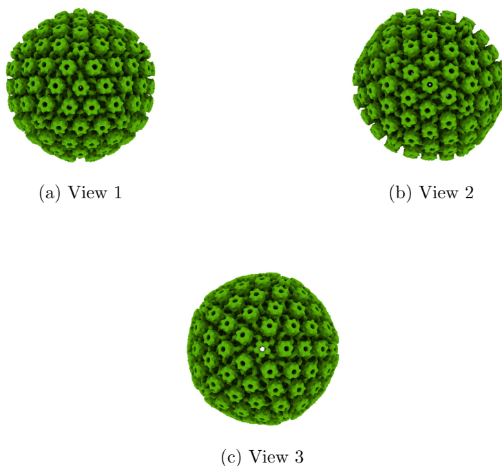
Figure 4: Isosurface at threshold=0.030000. Views generated by ChimeraX at the following X, Y, Z angles: View 1 (0, -90, -90), View 2 (-90, 0, -90), View 3 (0, 0, 0).
