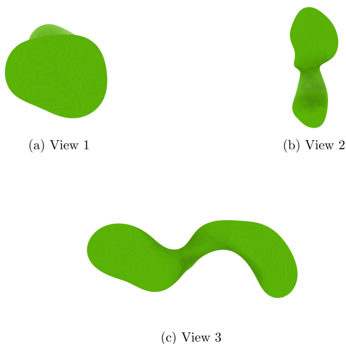
Figure 4: Isosurface at threshold=0.800000. Views generated by ChimeraX at a the following X, Y, Z angles: View 1 (0, -90, -90), View 2 (-90, 0, -90), View 3 (0, 0, 0).
