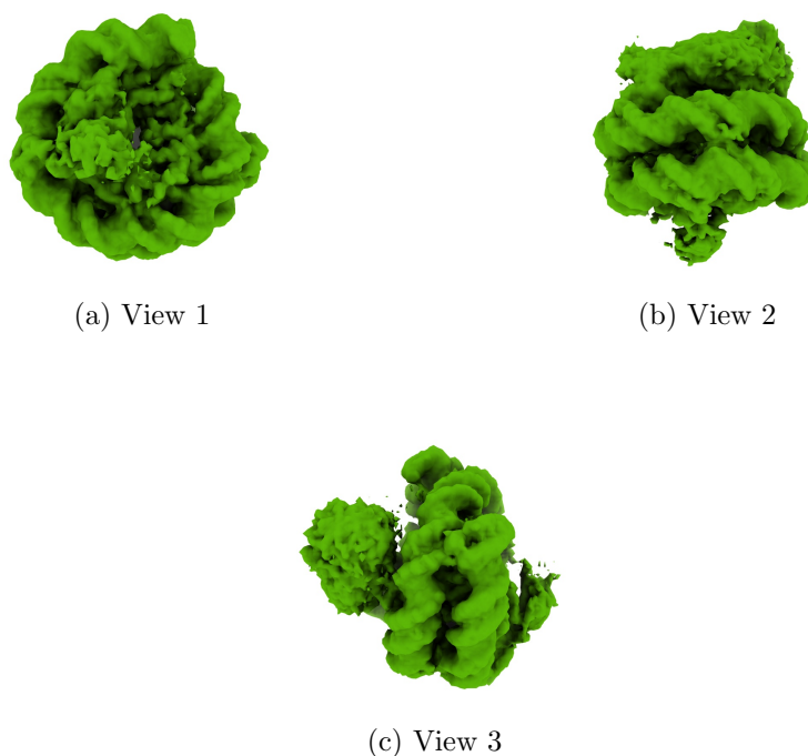
Figure 4: Isosurface at threshold=3.600000. Views generated by ChimeraX at a the following X, Y, Z angles: View 1 (0, -90, -90), View 2 (-90, 0, -90), View 3 (0, 0, 0).
