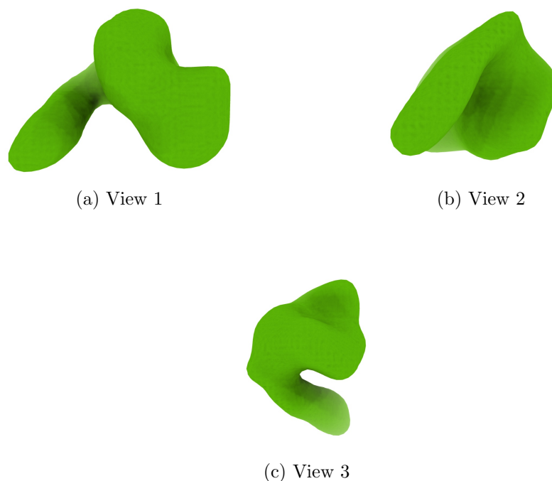
Figure 4: Isosurface at threshold=0.844000. Views generated by ChimeraX at a the following X, Y, Z angles: View 1 (0, -90, -90), View 2 (-90, 0, -90), View 3 (0, 0, 0).
