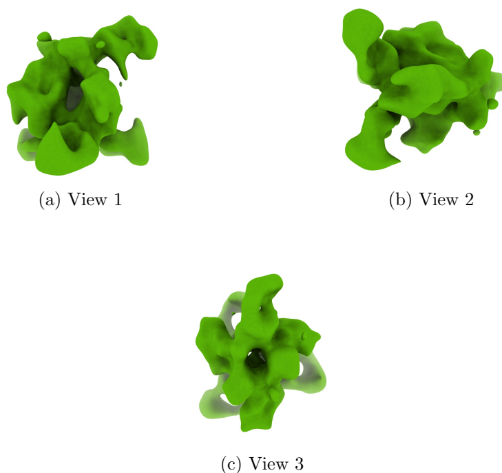
Figure 4: Isosurface at threshold=0.015000. Views generated by ChimeraX at the following X, Y, Z angles: View 1 (0, -90, -90), View 2 (-90, 0, -90), View 3 (0, 0, 0).
