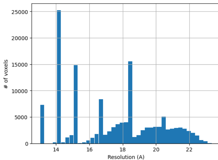
Figure 21: Histogram of the local resolution according to MonoRes.
