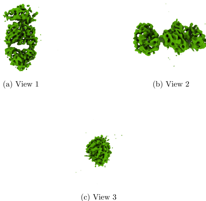
Figure 4: Isosurface at threshold=3.400000. Views generated by ChimeraX at a the following X, Y, Z angles: View 1 (0, -90, -90), View 2 (-90, 0, -90), View 3 (0, 0, 0).
