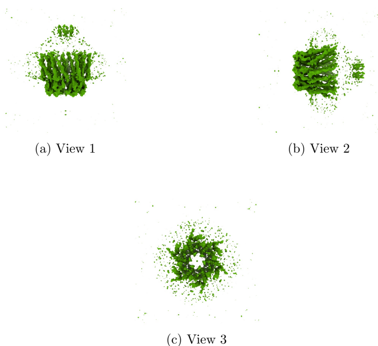
Figure 4: Isosurface at threshold=0.510000. Views generated by ChimeraX at a the following X, Y, Z angles: View 1 (0, -90, -90), View 2 (-90, 0, -90), View 3 (0, 0, 0).
