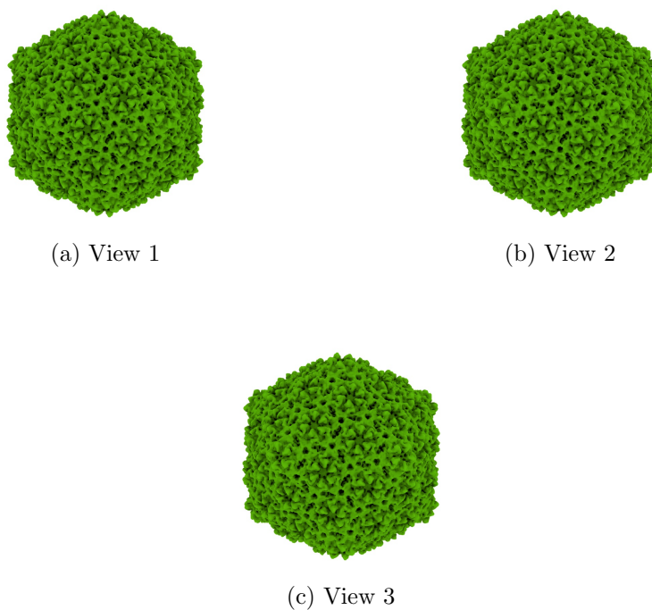
Figure 4: Isosurface at threshold=1892.000000. Views generated by ChimeraX at a the following X, Y, Z angles: View 1 (0, -90, -90), View 2 (-90, 0, -90), View 3 (0, 0, 0).
