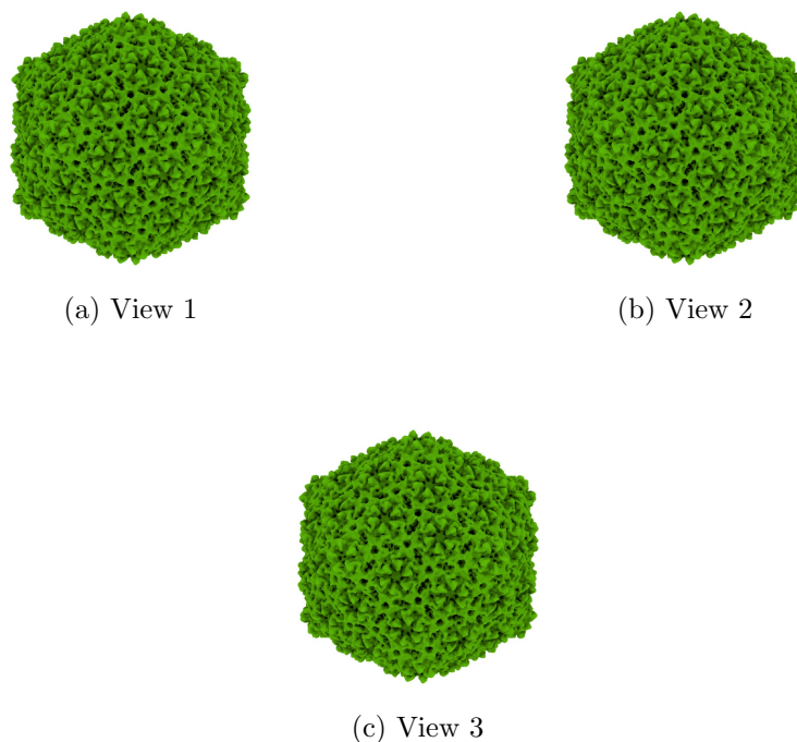
Figure 4: Isosurface at threshold=1892.000000. Views generated by ChimeraX at the following X, Y, Z angles: View 1 (0, -90, -90), View 2 (-90, 0, -90), View 3 (0, 0, 0).
