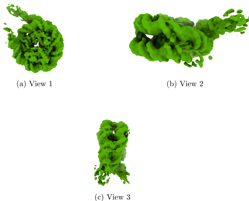
Figure 4: Isosurface at threshold=0.310000. Views generated by ChimeraX at a the following X, Y, Z angles: View 1 (0, -90, -90), View 2 (-90, 0, -90), View 3 (0, 0, 0).
