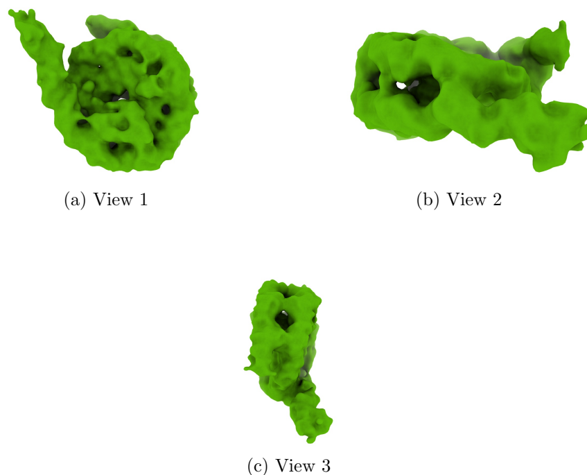
Figure 4: Isosurface at threshold=0.017000. Views generated by ChimeraX at a the following X, Y, Z angles: View 1 (0, -90, -90), View 2 (-90, 0, -90), View 3 (0, 0, 0).
