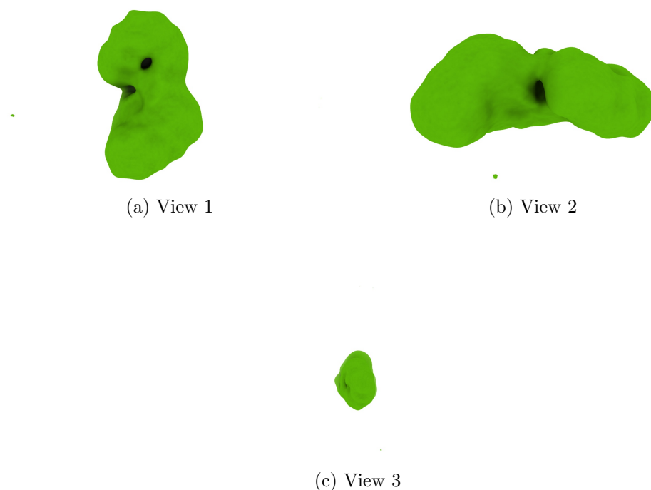
Figure 4: Isosurface at threshold=0.309000. Views generated by ChimeraX at a the following X, Y, Z angles: View 1 (0, -90, -90), View 2 (-90, 0, -90), View 3 (0, 0, 0).
