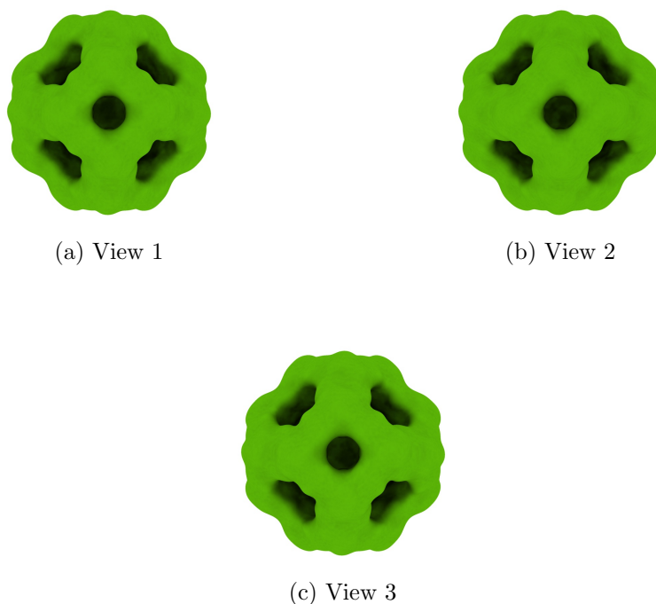
Figure 4: Isosurface at threshold=1.800000. Views generated by ChimeraX at a the following X, Y, Z angles: View 1 (0, -90, -90), View 2 (-90, 0, -90), View 3 (0, 0, 0).
