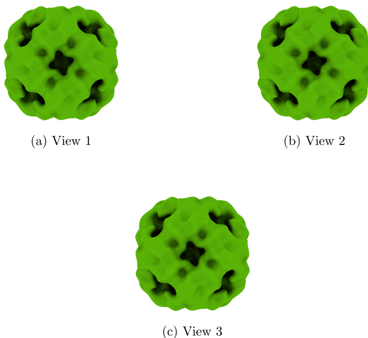
Figure 4: Isosurface at threshold=2.310000. Views generated by ChimeraX at a the following X, Y, Z angles: View 1 (0, -90, -90), View 2 (-90, 0, -90), View 3 (0, 0, 0).
