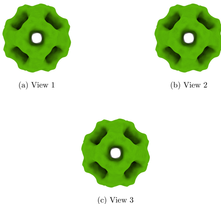
Figure 4: Isosurface at threshold=2.120000. Views generated by ChimeraX at a the following X, Y, Z angles: View 1 (0, -90, -90), View 2 (-90, 0, -90), View 3 (0, 0, 0).
