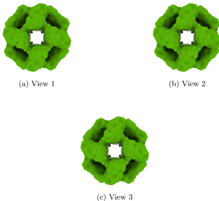
Figure 4: Isosurface at threshold=2.410000. Views generated by ChimeraX at a the following X, Y, Z angles: View 1 (0, -90, -90), View 2 (-90, 0, -90), View 3 (0, 0, 0).
