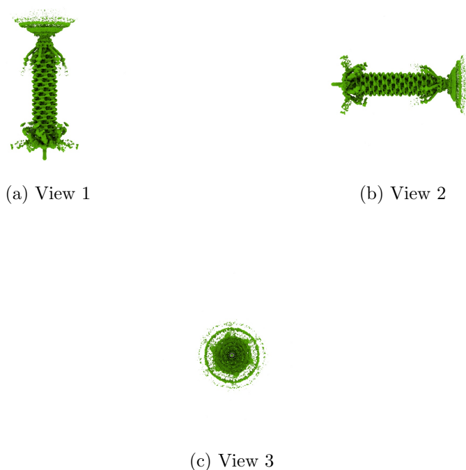
Figure 4: Isosurface at threshold=2.700000. Views generated by ChimeraX at a the following X, Y, Z angles: View 1 (0, -90, -90), View 2 (-90, 0, -90), View 3 (0, 0, 0).
