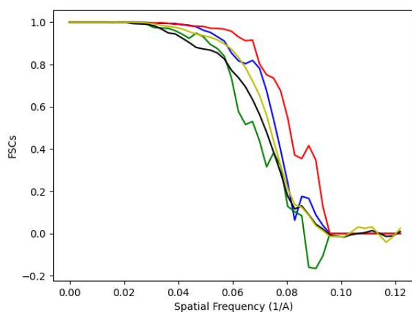
Figure 25: FSC in X, Y, Z, the global FSC, and the Average Cosine Phase.
