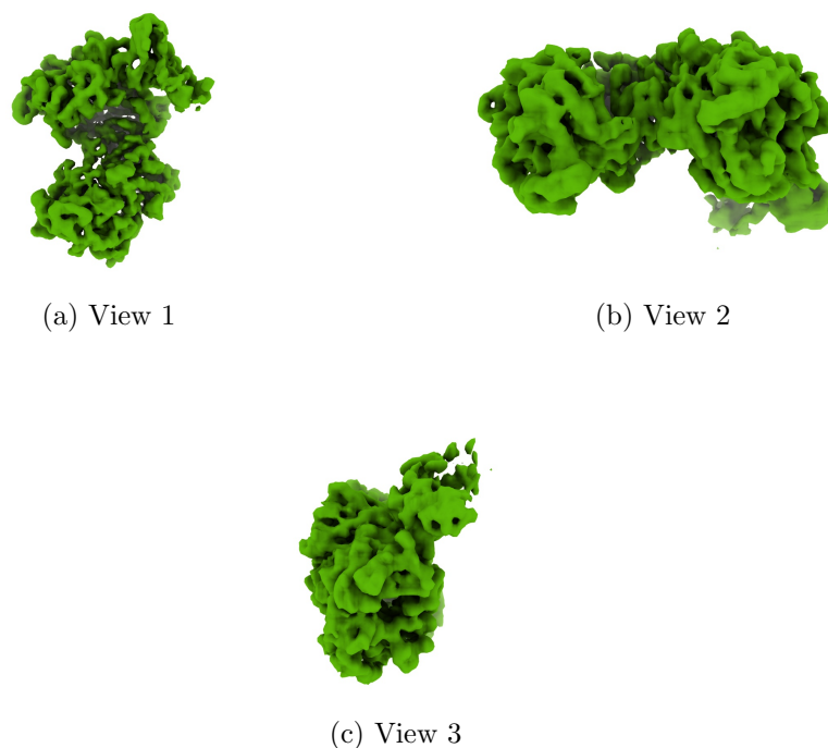
Figure 4: Isosurface at threshold=0.063900. Views generated by ChimeraX at a the following X, Y, Z angles: View 1 (0, -90, -90), View 2 (-90, 0, -90), View 3 (0, 0, 0).
