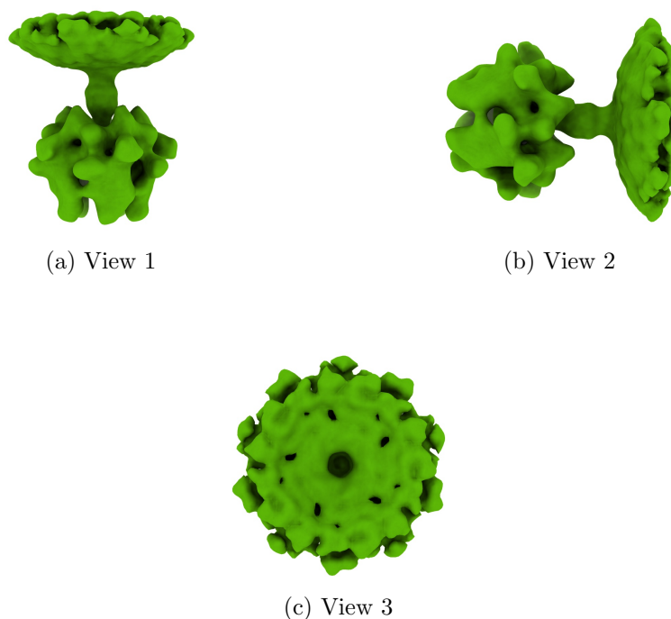
Figure 4: Isosurface at threshold=0.012000. Views generated by ChimeraX at the following X, Y, Z angles: View 1 (0, -90, -90), View 2 (-90, 0, -90), View 3 (0, 0, 0).
