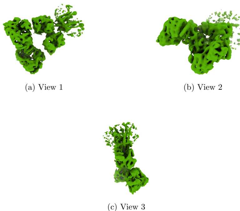
Figure 4: Isosurface at threshold=0.358000. Views generated by ChimeraX at a the following X, Y, Z angles: View 1 (0, -90, -90), View 2 (-90, 0, -90), View 3 (0, 0, 0).
