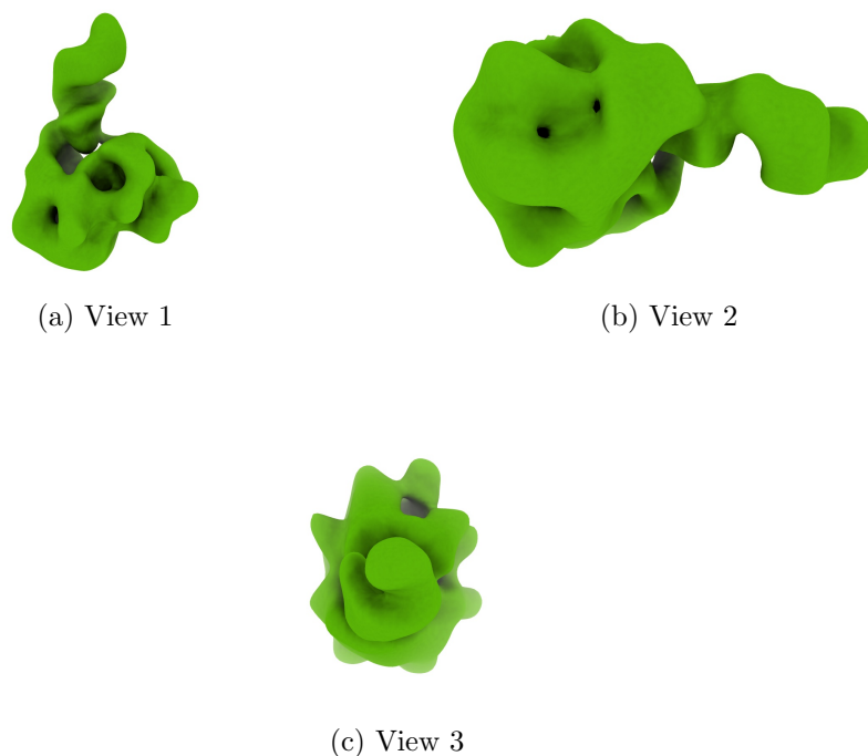
Figure 4: Isosurface at threshold=0.324000. Views generated by ChimeraX at a the following X, Y, Z angles: View 1 (0, -90, -90), View 2 (-90, 0, -90), View 3 (0, 0, 0).
