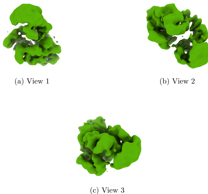
Figure 4: Isosurface at threshold=1.690000. Views generated by ChimeraX at a the following X, Y, Z angles: View 1 (0, -90, -90), View 2 (-90, 0, -90), View 3 (0, 0, 0).
