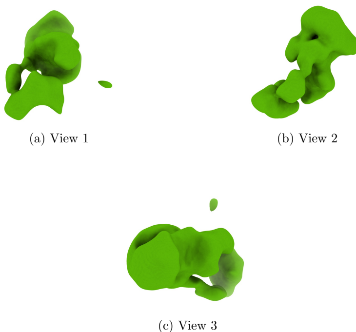
Figure 4: Isosurface at threshold=2.400000. Views generated by ChimeraX at a the following X, Y, Z angles: View 1 (0, -90, -90), View 2 (-90, 0, -90), View 3 (0, 0, 0).
