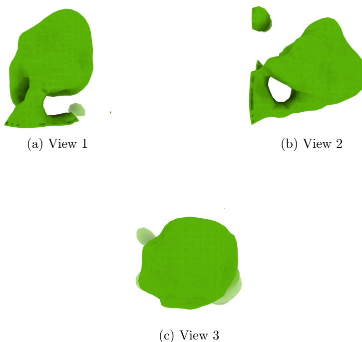
Figure 4: Isosurface at threshold=0.044200. Views generated by ChimeraX at a the following X, Y, Z angles: View 1 (0, -90, -90), View 2 (-90, 0, -90), View 3 (0, 0, 0).
