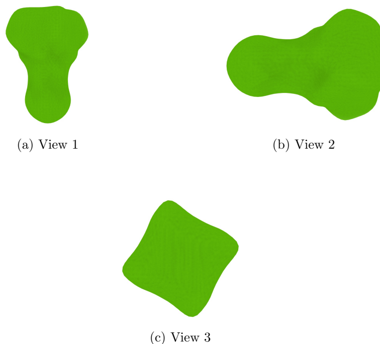
Figure 4: Isosurface at threshold=2.890000. Views generated by ChimeraX at a the following X, Y, Z angles: View 1 (0, -90, -90), View 2 (-90, 0, -90), View 3 (0, 0, 0).
