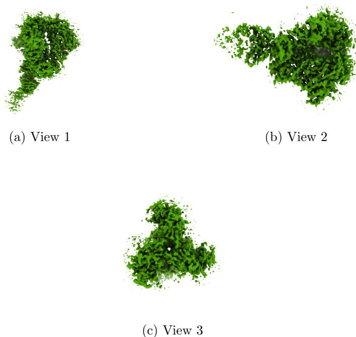
Figure 4: Isosurface at threshold=0.021000. Views generated by ChimeraX at a the following X, Y, Z angles: View 1 (0, -90, -90), View 2 (-90, 0, -90), View 3 (0, 0, 0).
