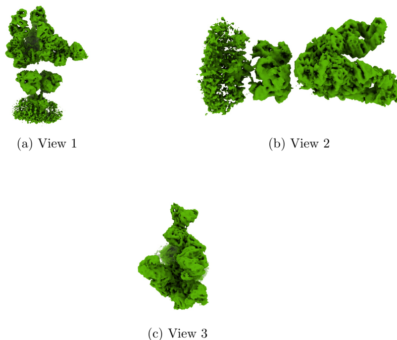
Figure 4: Isosurface at threshold=0.110000. Views generated by ChimeraX at a the following X, Y, Z angles: View 1 (0, -90, -90), View 2 (-90, 0, -90), View 3 (0, 0, 0).
