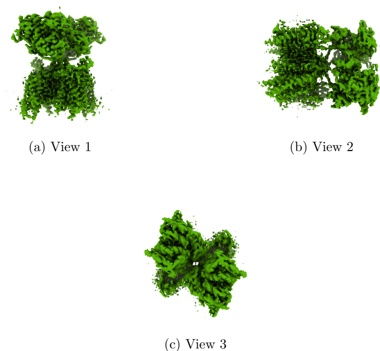
Figure 4: Isosurface at threshold=0.156000. Views generated by ChimeraX at a the following X, Y, Z angles: View 1 (0, -90, -90), View 2 (-90, 0, -90), View 3 (0, 0, 0).
