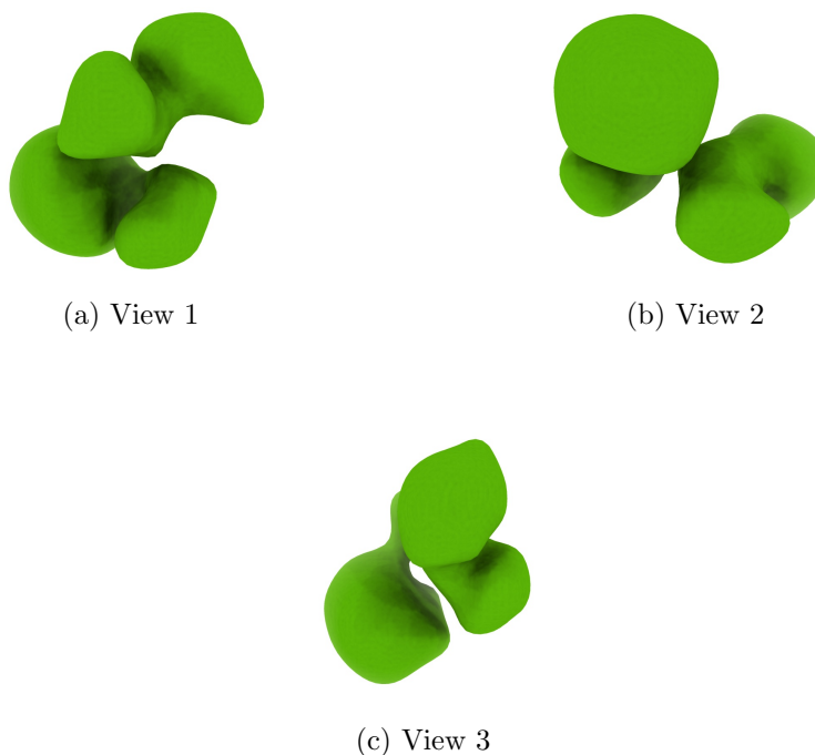
Figure 4: Isosurface at threshold=0.038100. Views generated by ChimeraX at a the following X, Y, Z angles: View 1 (0, -90, -90), View 2 (-90, 0, -90), View 3 (0, 0, 0).
