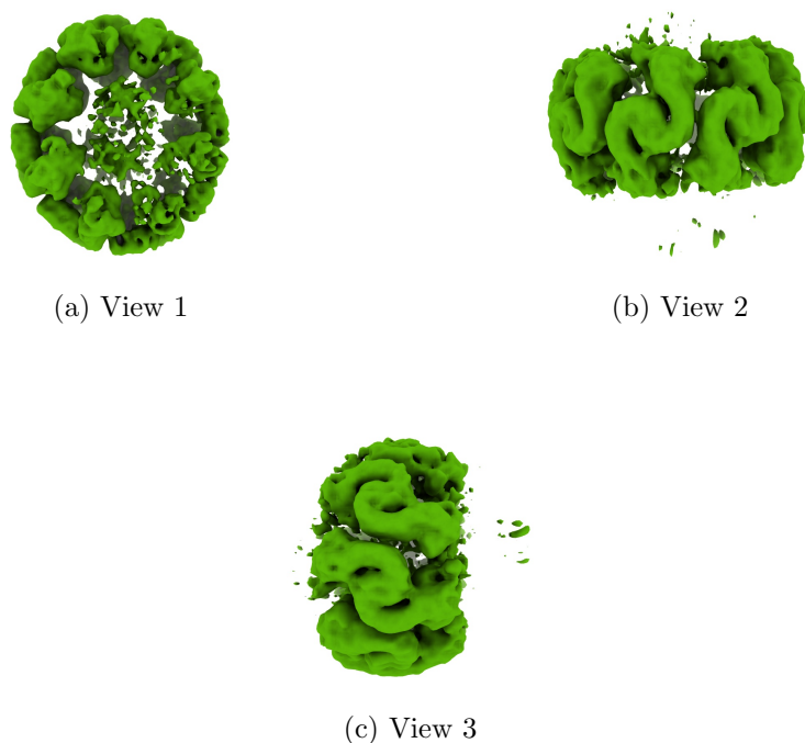
Figure 4: Isosurface at threshold=0.343000. Views generated by ChimeraX at a the following X, Y, Z angles: View 1 (0, -90, -90), View 2 (-90, 0, -90), View 3 (0, 0, 0).
