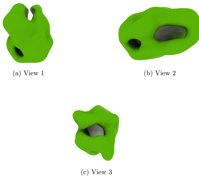
Figure 4: Isosurface at threshold=3.230000. Views generated by ChimeraX at a the following X, Y, Z angles: View 1 (0, -90, -90), View 2 (-90, 0, -90), View 3 (0, 0, 0).
