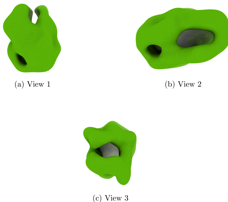
Figure 4: Isosurface at threshold=3.230000. Views generated by ChimeraX at the following X, Y, Z angles: View 1 (0, -90, -90), View 2 (-90, 0, -90), View 3 (0, 0, 0).
